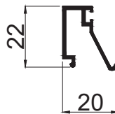
SINGLE GLASS CLIP (5mm Glass Thick) CODE - Z29CLP WEIGHT KG/M - 0.230
