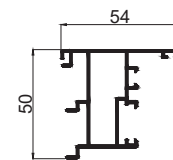
FLYING MULLION CODE -C0C04M WEIGHT KG/M - 0.911
