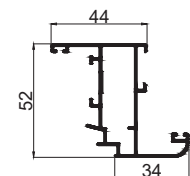
WINDOW OPEN - IN SHUTTER CODE - CC03EM WEIGHT KG/M - 0.947
