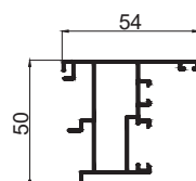
FLYING MULLION CODE - C0C04M WEIGHT KG/M - 0.911
