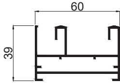
GEETA 2 TRACK 25 X 54 WITH LEG CODE - G2L255 WEIGHT KG/M - 1.000
