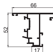
WINDOW OPEN - OUT SHUTTER CODE - C0C07M WEIGHT KG/M - 1.094
