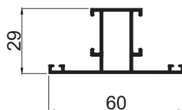
MULLION CODE - Z29MUL WEIGHT KG/M - 0.600
