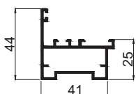
INVERSION CLIP CODE - C0C18M WEIGHT KG/M - 0.745
