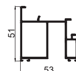
DOOR BOTTOM CLIP (FOR AUTO DROP SEAL) CODE - WEIGHT KG/M - 0.915
