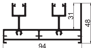
ADDON 2 TRACK TOP BOTTOM CODE - G382TB WEIGHT KG/M - 1.852
