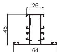
WINDOW MULLION CODE - C0C02M WEIGHT KG/M - 0.917
