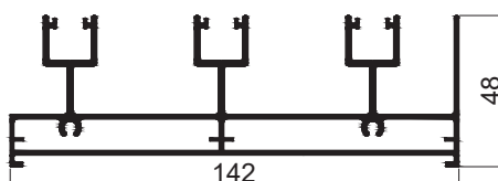
ADD ON 3 TRACK TOP BOTTOM CODE - G383TB WEIGHT KG/M - 2.220
