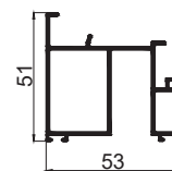
DOOR BOTTOM CLIP (FOR AUTO DROP SEAL) CODE - WEIGHT KG/M - 0.915
