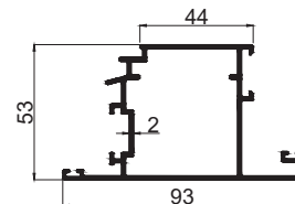
DOOR OPEN - OUT SHUTTER CODE - CM04AM WEIGHT KG/M - 1.500
