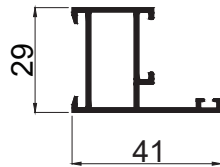
OUTER FRAME CODE - Z29FRM WEIGHT KG/M - 0.500
