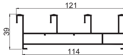
FRAME 4 TRACK CODE - G42554 WEIGHT KG/M - 1.650
