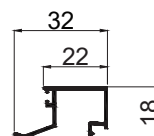
SINGLE GLASS CLIP ( 6mm,8mmGlass Thick ) CODE - Z40SGC WEIGHT KG/M - 0.250
