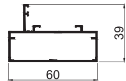
GEETA OUTER FRAME 25 X54 2L CODE - GF2L25 WEIGHT KG/M - 0.770
