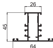
WINDOW MULLION CODE - C0C02M WEIGHT KG/M - 0.917
