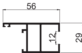
SHUTTER CODE - Z29STR WEIGHT KG/M - 0.640
