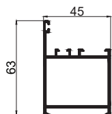
DOOR OUTER FRAME CODE - C0M01M WEIGHT KG/M - 1.129
