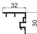
REGULER INTERLOCK CODE - GIW255 WEIGHT KG/M - 0.370
