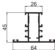
WINDOW MULLION CODE - C0C02M WEIGHT KG/M - 0.917
