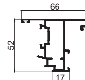
WINDOW OPEN - OUT SHUTTER CODE - C0C07M WEIGHT KG/M - 1.094
