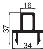
MEETING CODE - GM2554 WEIGHT KG/M - 0.215
