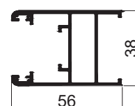
DOUBLE GLASS SHUTTER CODE - G3800S WEIGHT KG/M - 1.100
