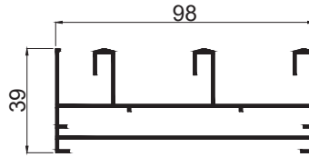
GEETA 3 TRACK 25 X 54 WITH LEG CODE - G3L255 WEIGHT KG/M - 1.450
