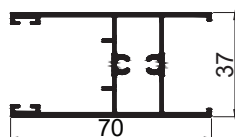
DGU SHUTTER TOP BOTTOM CODE - G38BTB WEIGHT KG/M - 1.06
