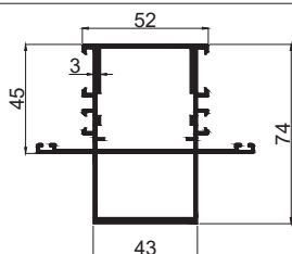
REINFORCEMENT MULLION CODE - CC02BM WEIGHT KG/M - 2.017
