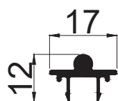
GUIDE RAIL CODE - C8A17M WEIGHT KG/M - 0.159
