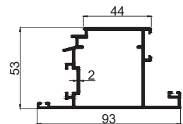
DOOR OPEN - OUT SHUTTER CODE - CM04AM WEIGHT KG/M - 1.500
