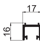
BOTTOM ADAPTOR CODE - C8006M WEIGHT KG/M - 0.259
