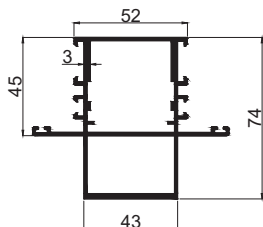
REINFORCEMENT MULLION CODE - CC02BM WEIGHT KG/M - 2.017
