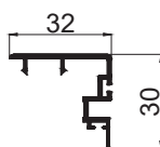
REGULER INTERLOCK CODE - GIW255 WEIGHT KG/M - 0.370
