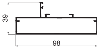
GEETA OUTER FRAME 25 X54 3L CODE - GF3L25 WEIGHT KG/M - 1.170
