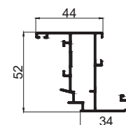
WINDOW OPEN - IN SHUTTER CODE - CC03EM WEIGHT KG/M - 0.947
