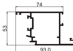
DOOR OPEN - IN SHUTTER CODE - CM03AM WEIGHT KG/M - 1.396
