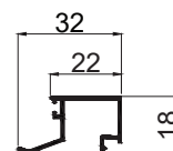
SINGLE GLASS CLIP ( 6mm,8mmGlass Thick ) CODE - Z40SGC WEIGHT KG/M - 0.250
