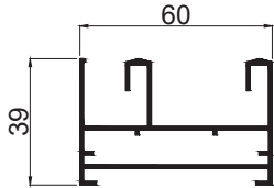
GEETA 2 TRACK 25 X 54 WITH LEG CODE - G2L255 WEIGHT KG/M - 1.000
