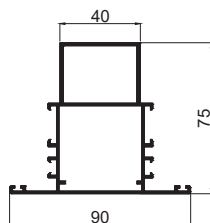
REINFORCEMENT MULLION-R CODE - WEIGHT KG/M - 1.450
