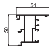
FLYING MULLION CODE -C0C04M WEIGHT KG/M - 0.911
