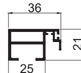
SLIM INTERLOCK (NON KPA) CODE - GI2554 WEIGHT KG/M - 0.530
