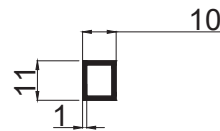
11.2X9.5MM TUBE CODE - GBFLTU WEIGHT KG/M - 0.150
