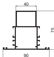
REINFORCEMENT MULLION-R CODE - WEIGHT KG/M - 1.450
